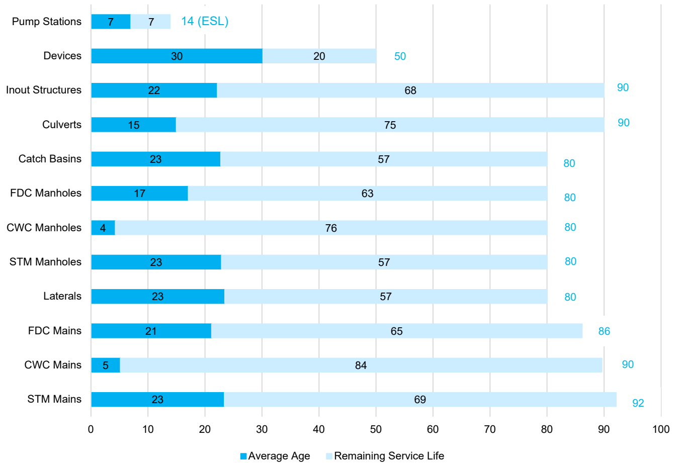
Figure 5-1: Average Asset Age as a Proportion of Average Expected Service Life (Stormwater Services)
