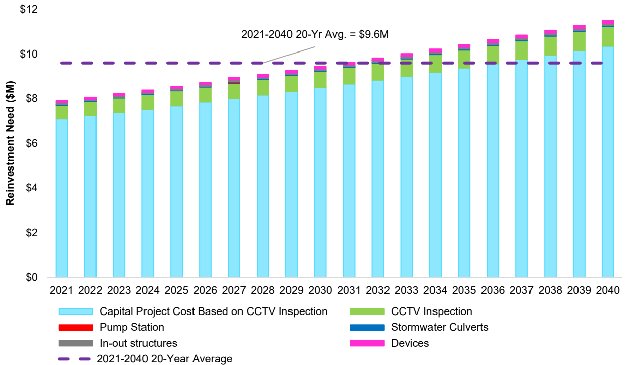
Figure 5-9: Stormwater 20-Year Reinvestment Need Details
