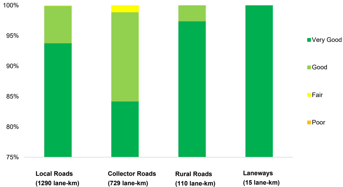
Figure 6-4: Asset Condition Detail (Road Services)
