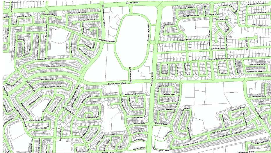
Figure 2-5: Thiessen Polygons Modeling- A Sample
